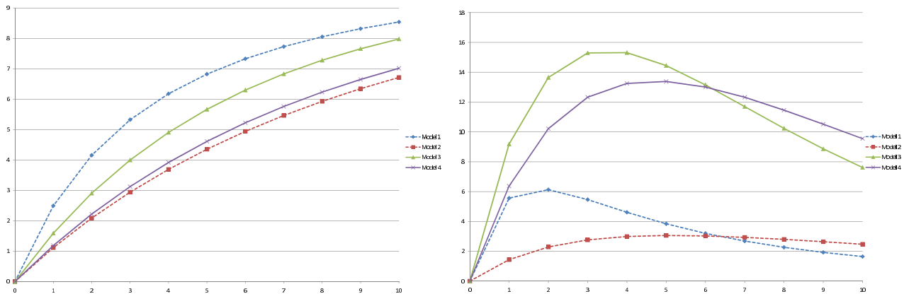
Figure 1: Evolution of \mathbb{E}[N_t] (left) and \mathbb{V}[N_t] (right) as a function of t , for all the models described in Definition 4.1. The curves plotted with dotted lines correspond to the case where direct defaults are i.i.d.
