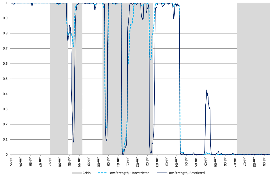
(a) Time-varying strength, constant structure
