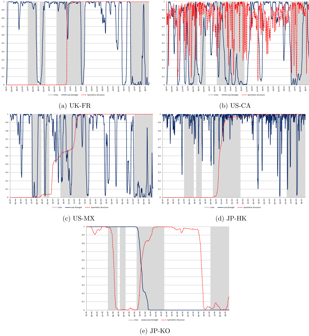
Figure 4: Smoothed inference probabilities for other country pairs
