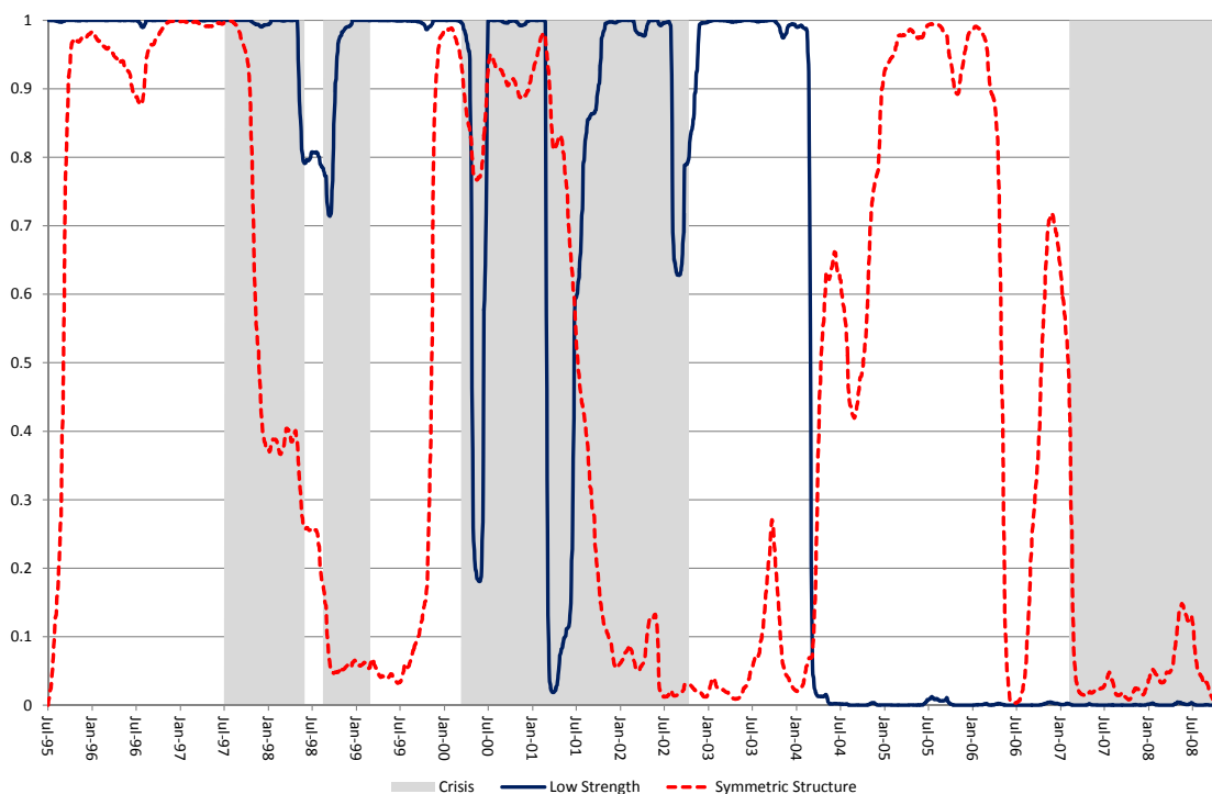
Figure 2: Smoothed inference probabilities for UK-GE
