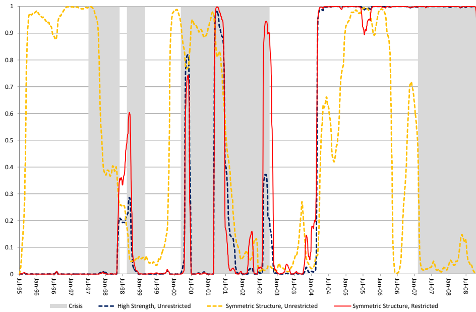
(b) Constant strength, time-varying structure
