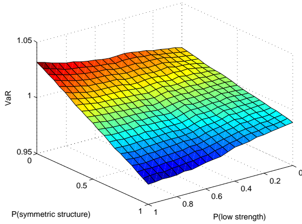
(a) UK-GE – Strength regimes only
