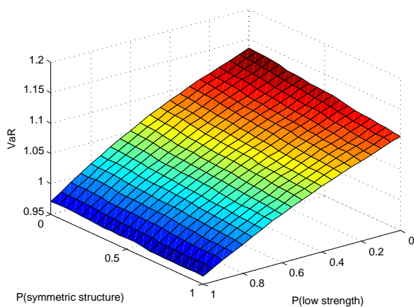
(j) JP-HK – Structure regimes only
