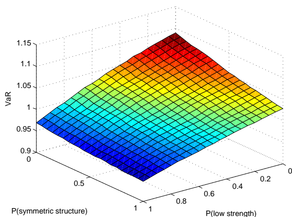
(h) US-MX – Structure regimes only
