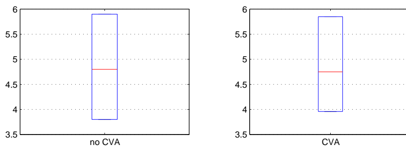
Figure 10: Distribution of the volumes of exposures without and with CVA surcharge
