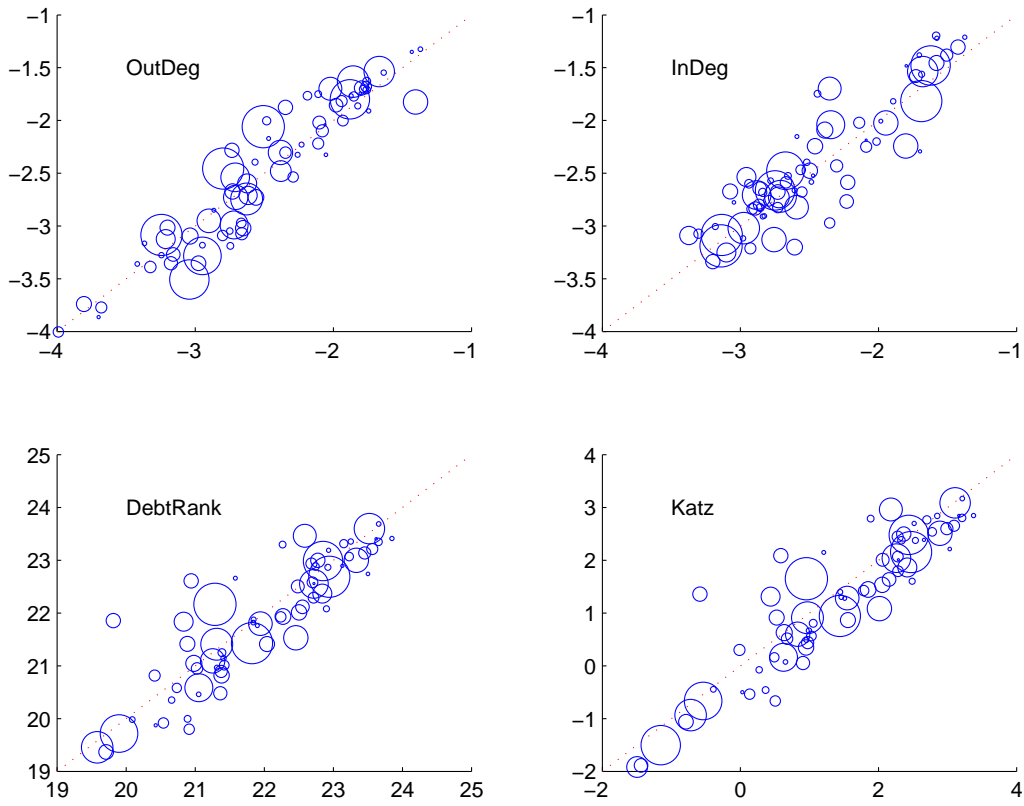
Figure 13: Impact of the adverse scenario on the interbank network structures
