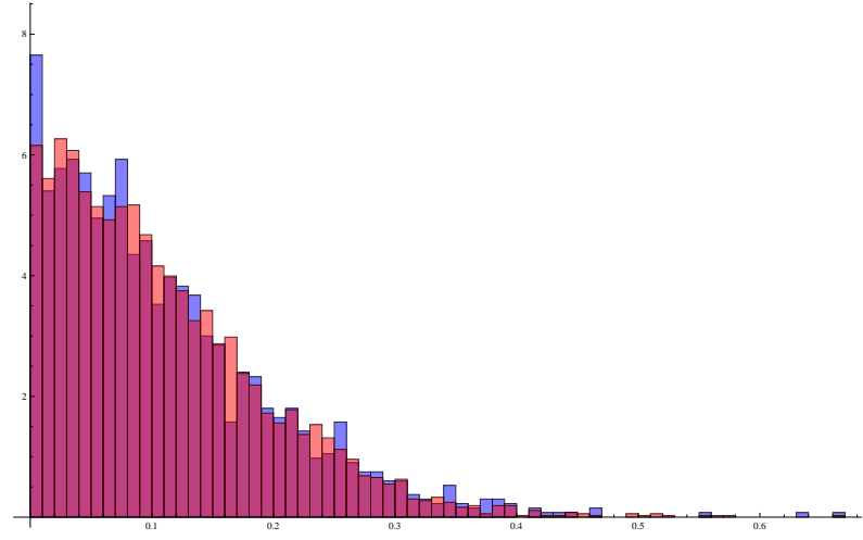
f. Autocorrelation
