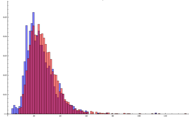
e. Volatility
