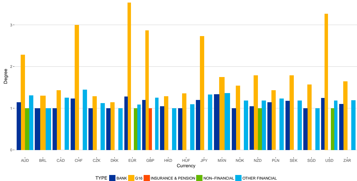
Figure 14: Average degree (number of counterparty relationships of a given institution) by currency in which the IRD constituting the counterparty relationship is denominated and type of institution, for the networks of central counterparties and their clearing members. Missing values due to no observations or confidentiality. In particular, CCPs are not shown due to confidentiality reasons. If CCPs were shown, they would be often an order of magnitude higher than the other categories. We would thus observe that all the richness of the full picture with client clearing is gone, and CCPs dominate this side of the clearing network. On the one hand, this underlies the importance of client clearing for analysing full implications of interconnectedness in this market, but on the other hand it also shows that we need to stress that CCPs remain the major contributors to the structure of this system.
